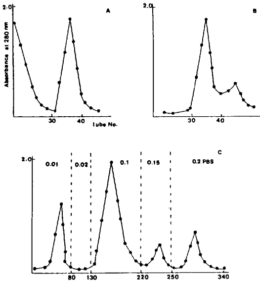
Fig. 3. CM-cellulose column chromatography of fractions of supernatant after centrifugation and eluted by PB (A) and stepwise (C); and fractions after Amberlite column and eluted by PB (B). Column size was 2.2 × 40cm. Flow rate was 3ml/min. Fraction volume was 5ml. The toxin was eluted with stepwise (0.01-0.2M PBS) and 0.2M PB.
