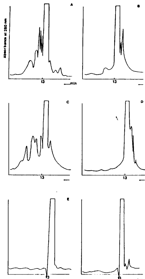
Fig. 6. FPLC of fractions after Amberlite CG-50 column (A); CM-column chromatography by PB elution (B); Amberlite IRC-50 column (C); CM-column chromatography by gradient (D); Standard as a reference (E); and after gel filtration on Ultro gel (F).
