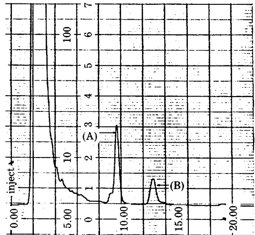
Fig. 6. Chromatogram of capsicum extract. Chromatographic condition: µ-Bondapak C 18 col; 45% acetonitrile in 0.3% phosphate, pH 4.0; flow rate, 1.2 ml/min; UV detection: 280 nm (A) Capsaicin; (B) Dihydrocapsaicin.
