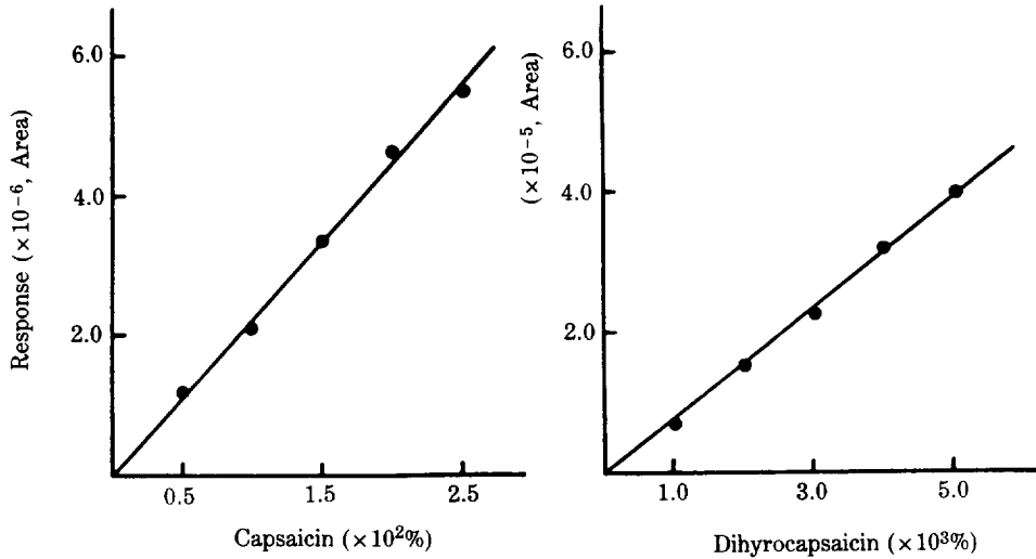
Fig. 2. Calibration curves of capsaicin and dihydrocapsaicin.
