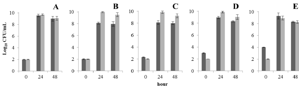
Fig. 3. Monitoring the number of L. monocytogenes (LM■) and L. innocua (LIN■) viable cells in LEB. Panel A: LM 10 2 CFU/mL LIN 10 2 CFU/mL culture. Panel B: mixed culture (LM 10 2 CFU/mL and LIN 10 2 CFU/mL) Panel C: mixed culture (LM 2.0 × 10 2 CFU/mL and LIN 10 2 CFU/mL). Panel D: mixed culture (LM 10 3 CFU/mL and LIN 10 2 CFU/mL). Panel E: mixed culture (LM 10 4 CFU/mL and LIN 10 2 CFU/mL).
